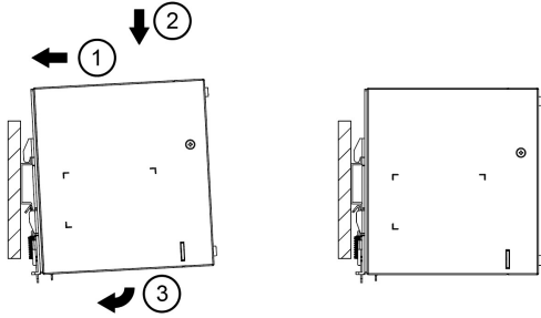
Fig. 3.1 Mounting
