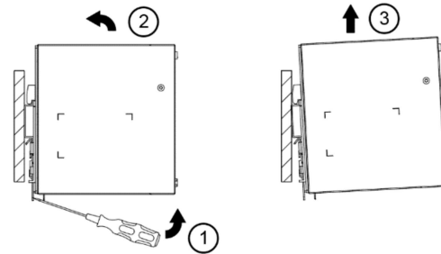
Fig. 3.2 Dismounting
